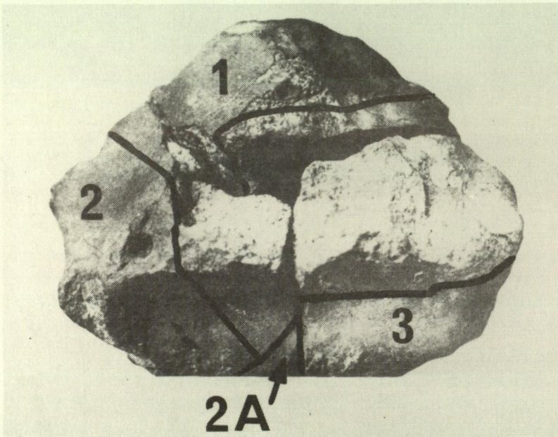
Fig. 2: Naretha meteorite. The photograph displayed with the W.A. School of Mines specimen and also used to illustrate 'Kingoonya' meteorite. Approximate limits of larger surviving fragments are shown on the front of the specimen only. Because of the flat obliquity of some cuts to the plane of the photograph, the material is more complete than might appear in this view. 1. W.A. School of Mines 3466. 2. Geological Survey of W.A. 1/4709. 2A. E.S. Simpson collection S.1177 (larger of the pieces), held in the W.A. Museum. 3. South Australian Museum G. 6062.
