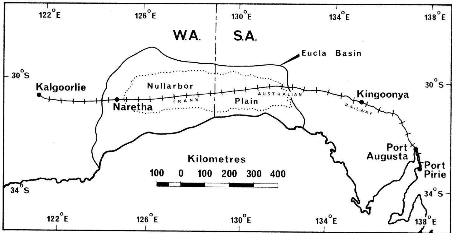
Fig. 1: Part of southern Australia showing Trans-Australian Railway in relation to Eucla Basin, Nullarbor Plain, and localities mentioned in text.
